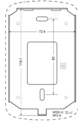
Drilling Template
